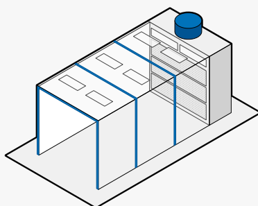
➤ Spray booth with canopy with walls and roof made of pre-insulated painted panels with lights
